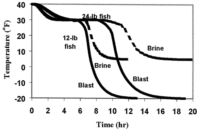
Figure 7. Compared performances of well-designed and operated blast and spray-brine freezers.
